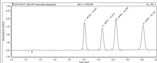
HPLC-UV chromatogram of Mix 5 (Aflatoxins) Lot # L19234M
