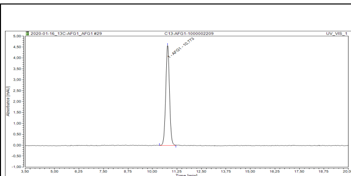
Figure 1: HPLC-UV chromatogram of U-[ 13 C 17 ]-Aflatoxin G1
